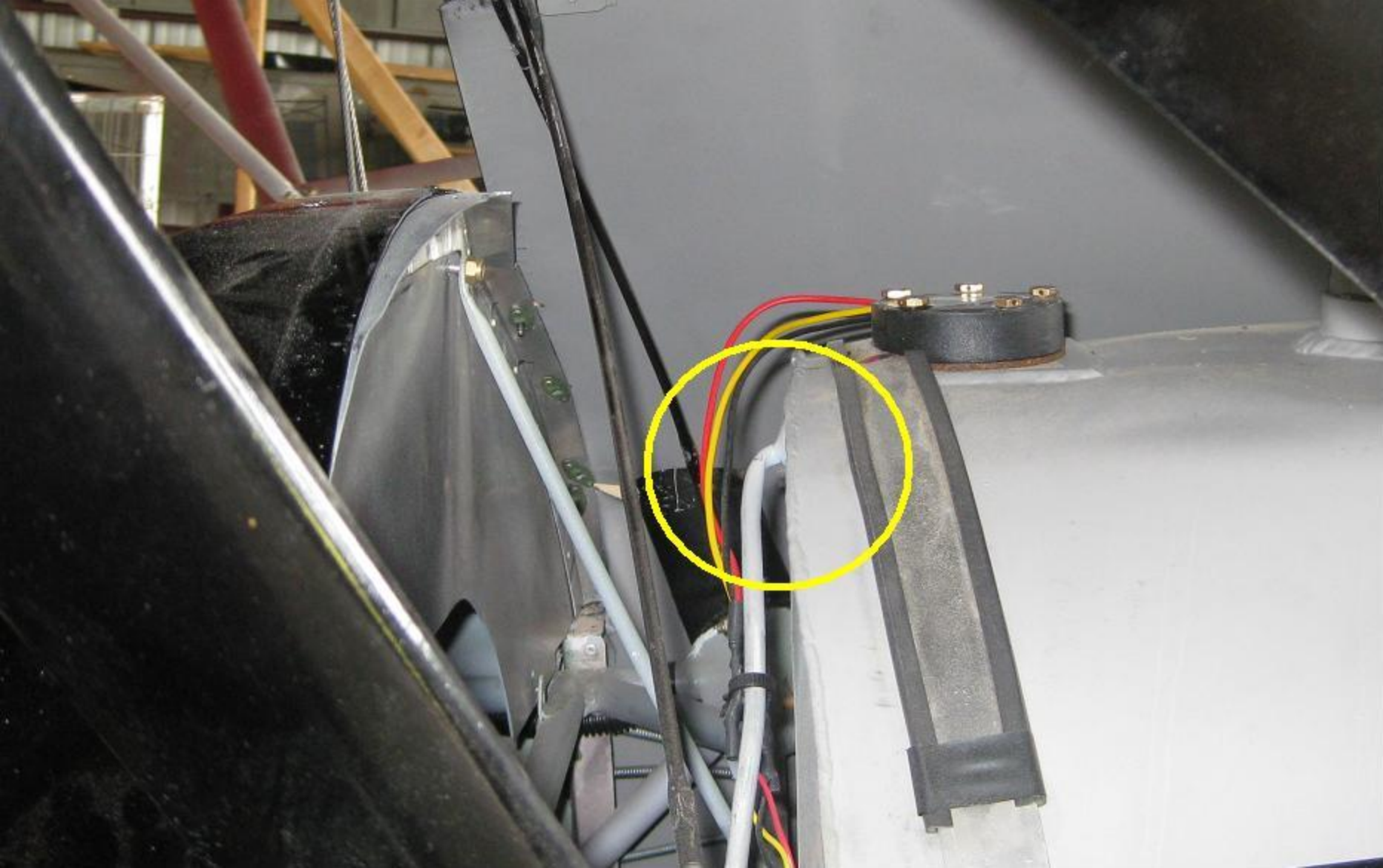
Photo 2. Crimped Fuel Vent.
